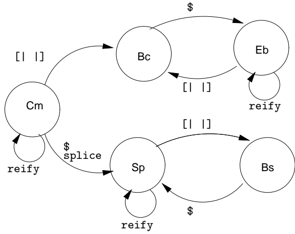
Figure 1. Typing states for Template Haskell
