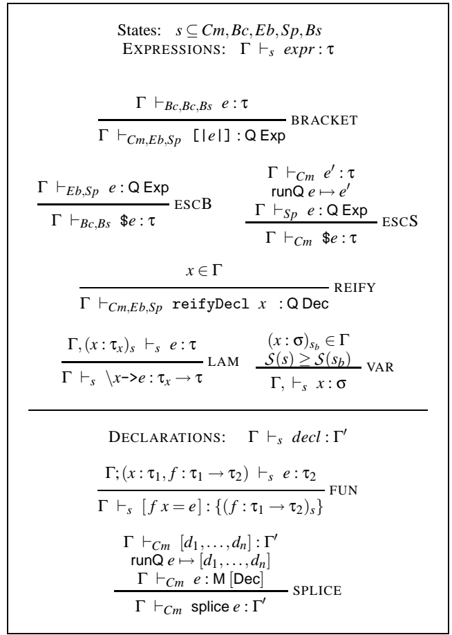
Figure 2. Typing rules for Template Haskell
